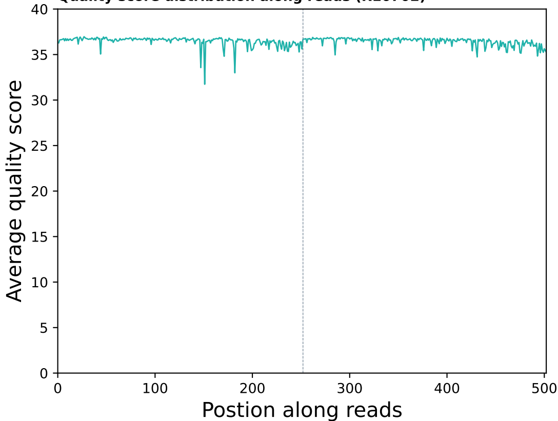
Quality score distribution along reads (R10702)
